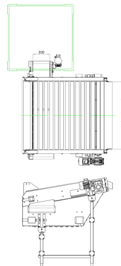
Plant view and side view of a small fruit eliminator
